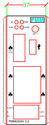
Front View
